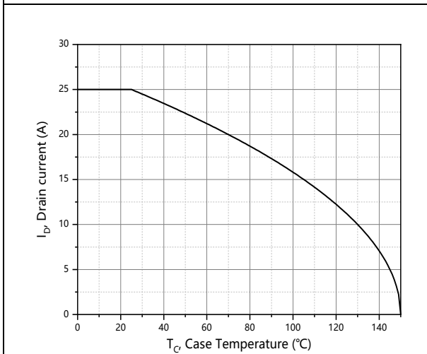
Figure 9. Drain current
